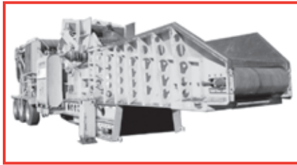
'99 CBI 4800 Grinder, 1677 Hrs., New Teeth, Updated Hammers, Full Engine Service, 12 Cyl. Diesel Engine, Stock #5134, Call.
